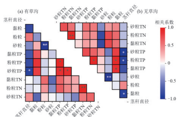
图 6 有、无草沟条件下各指标的相关关系 Fig. 6 Correlation among different indicators under conditions with and without grass ditches
